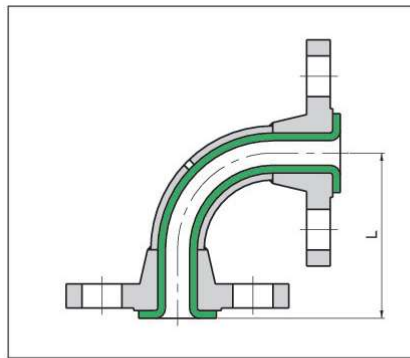
90° Steel Elbow
