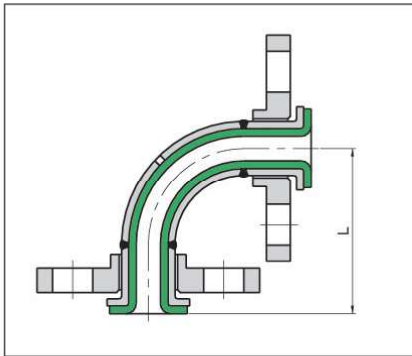
90° Stub-End Elbow
