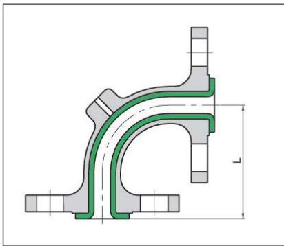
90° Cast Steel Elbow
