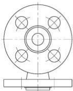
Orientation of Fixed Flange for 1" to 3" Sizes
