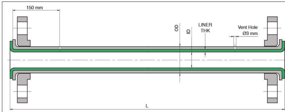
Stub-End Flange
