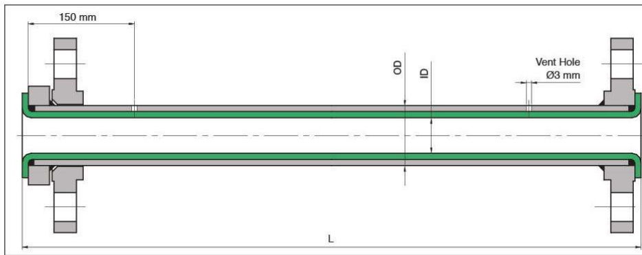
Fixed / Loose Flange
